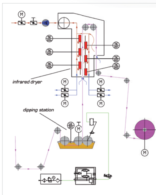
Coating process with IR dryer
